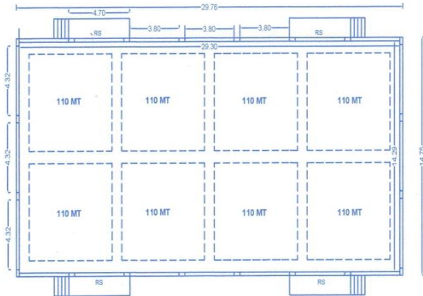
PLAN FOR 880 MT WH SCALE 1:100
