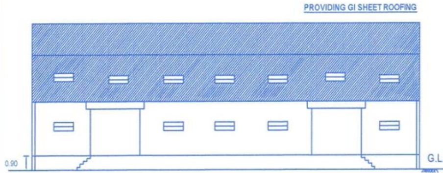
ELEVATION (WEST SIDE)
