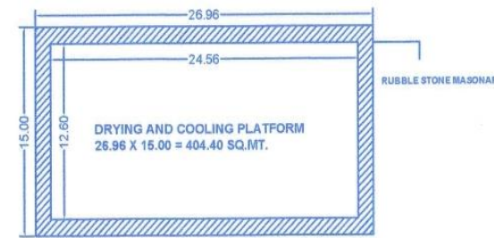
BUILT UP AREA OF DRYING AND COOLING PLATFORM
